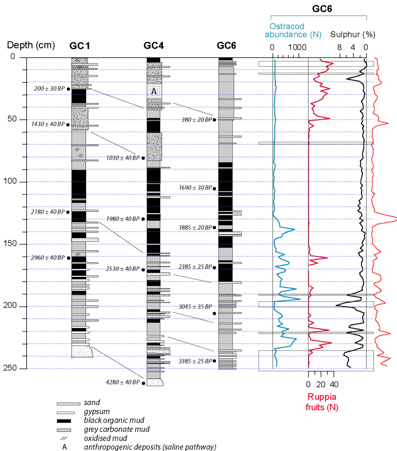
Figure 4. Lithostratigraphy and analytical data of GC1, GC4 and GC6 cores
