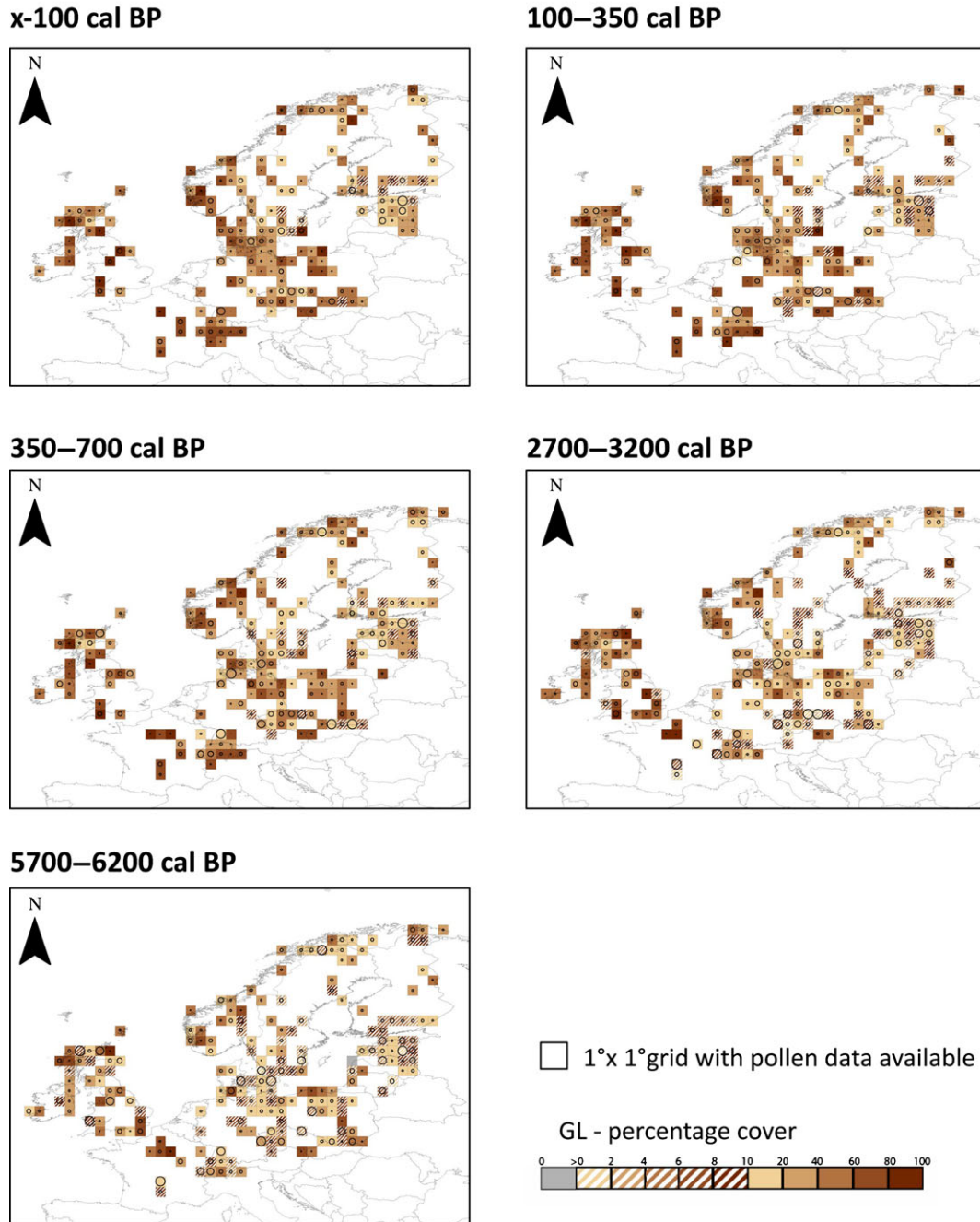
Fig. 4 Grid-based REVEALS estimates for the plant-functional type (PFT) grassland (GL) for five Holocene time-windows. For further figure interpretation, see Figs 2 and 3.
