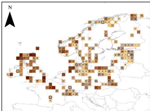
Fig. 2 Grid-based REVEALS estimates for the land-cover type (LCT) open land (OL) for the five Holocene time-windows. The scale is percentage cover, with the different colours indicating different percentage intervals: >0–10% in 2% intervals, 10–20% in a 10% interval, and 20–100% in 20% intervals. The category 0 (grey) corresponds to the grid cells with pollen records but no pollen for the actual LCT and, therefore, no REVEALS estimates. The category >0–2 corresponds to REVEALS estimates different from zero (can be less than 1%) up to 2%. The uncertainties of the LCTs and REVEALS estimates for the plant-functional types (PFTs) (Figs 3–5 and 8) are shown by circles of various sizes in each grid cell with a REVEALS estimate. The circles represent the coefficient of variation (CV; the standard error divided by the REVEALS estimate). When SE \geq REVEALS estimate, the circle fills the entire grid cell and the REVEALS estimate is considered unreliable. This occurs mainly where REVEALS estimates are low.
