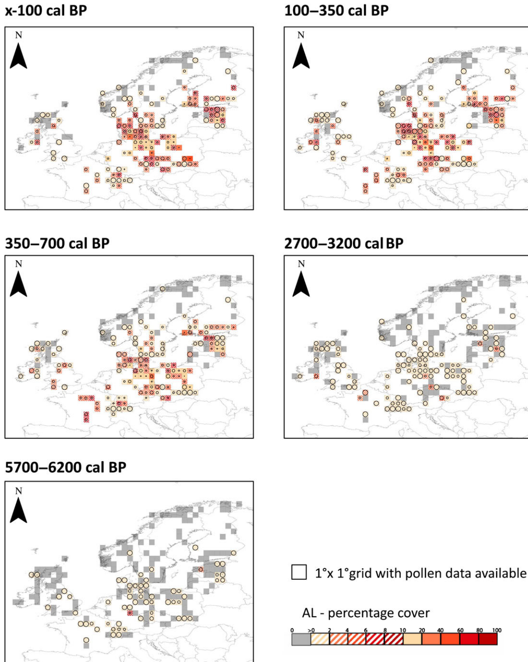
Fig. 3 Grid-based REVEALS estimates for the plant-functional type (PFTs) agricultural land (AL) for five Holocene time-windows. Grey-coloured grid cells (category 0) indicate that pollen data exist for those cells, but the actual PFT is not present in that specific time window. The uncertainties of the REVEALS estimates for the plant-functional types (PFTs) are shown in the same way as those for REVEALS LCTs (see Fig. 2). For further figure interpretation, see Fig. 2.
